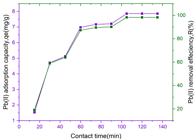
Fig. 10. Effect of contact on Pb (II) removal.
