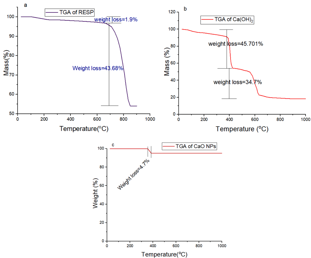
Fig. 5. TGA result: (a) Raw eggshell powder; (b) \text{Ca}(\text{OH})_2 gel; (c) CaO NPs.
