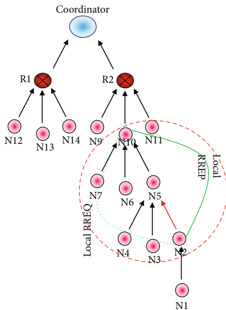
FIGURE 3: Data transmission via attacked region.
