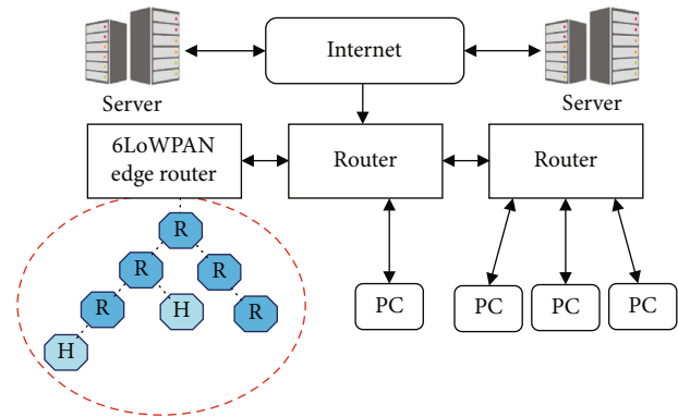
FIGURE 1: Schematic representation of the IPv6 transmission networks with a 6LoWPAN.
