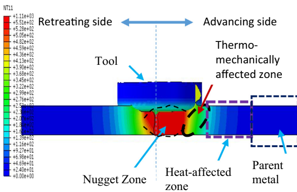
Fig. 8. Thermomechanical zone.
