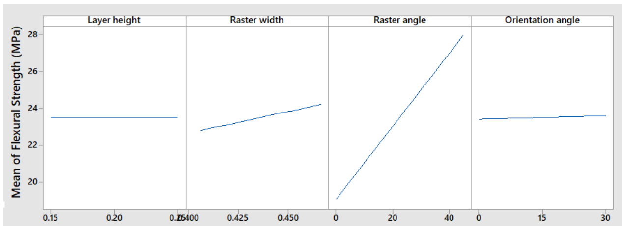
Figure 5. Factorial plots for flexural strength and inputs parameters.
