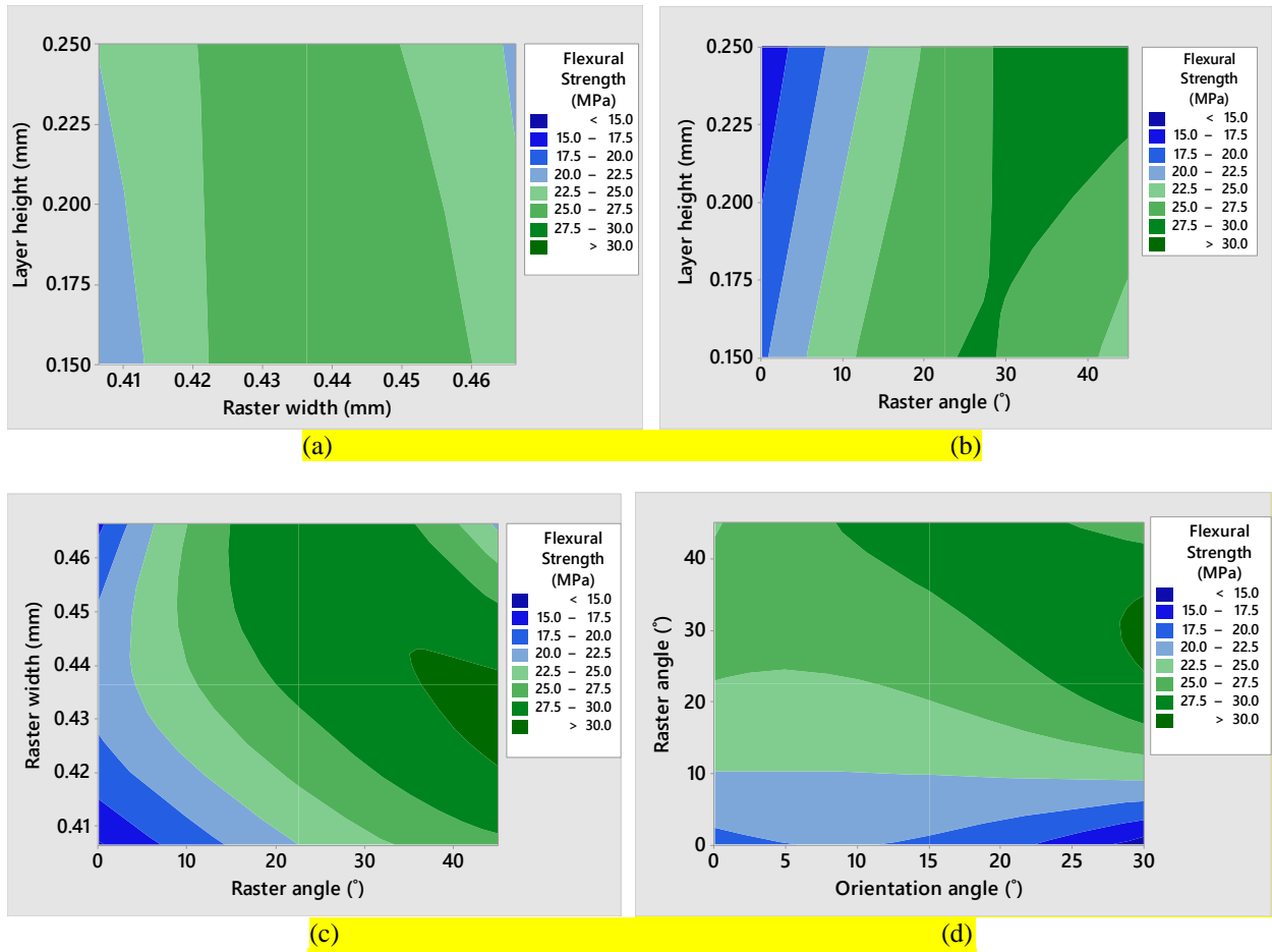
Figure 4. Contour plots of flexural strength with process parameters
