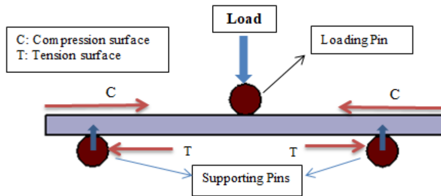
Figure 3. Experimental setup of flexural test
