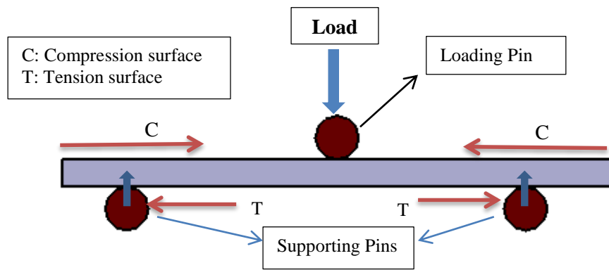
Figure 3. Experimental setup of flexural test
